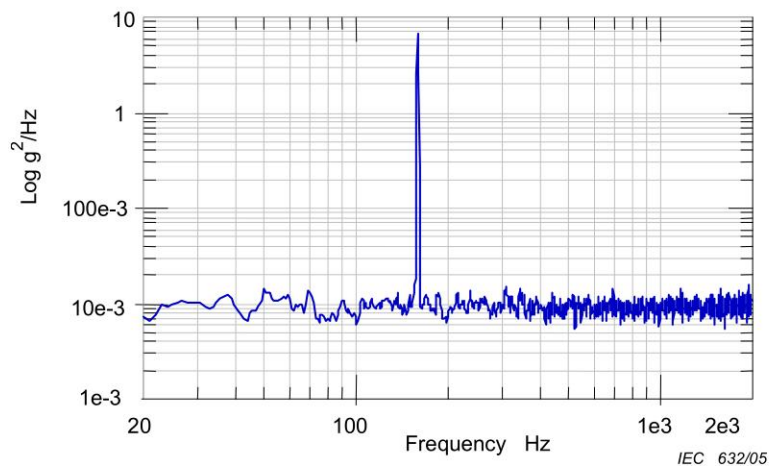
Figure A.1 – Sine at 160 Hz
