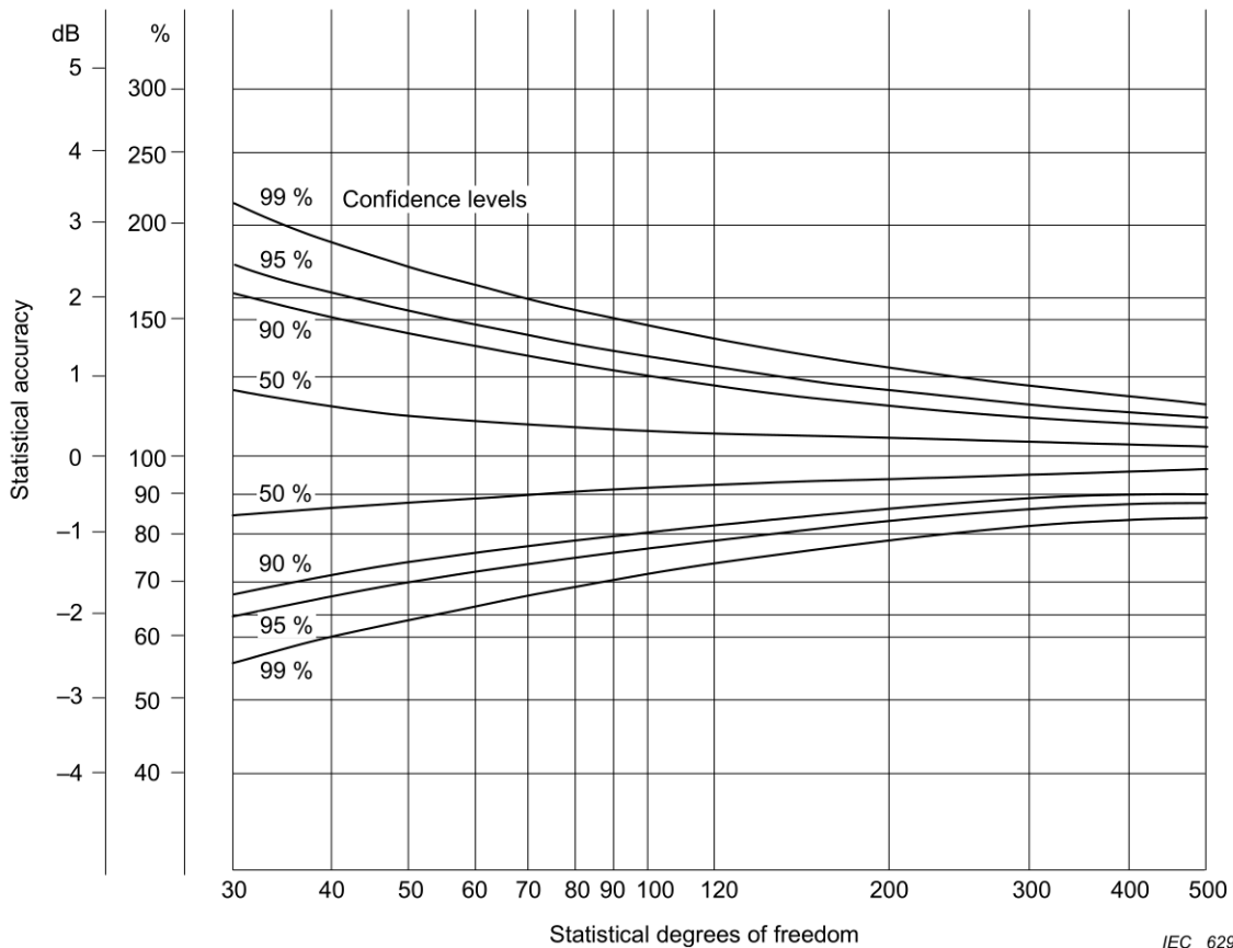
Figure 3 – Statistical accuracy of acceleration spectral density versus degrees of freedom for different confidence levels
