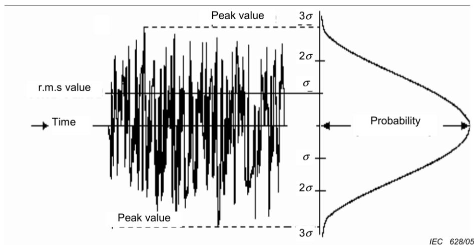
Figure 2 – Stochastic excitation, representation of signal clipping and Gaussian (normal) probability
